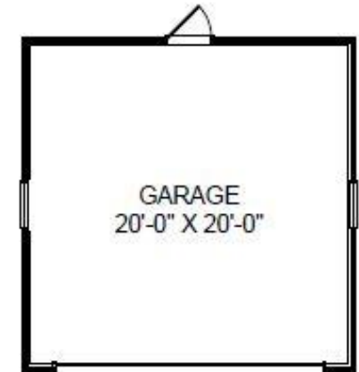
Garage Level
