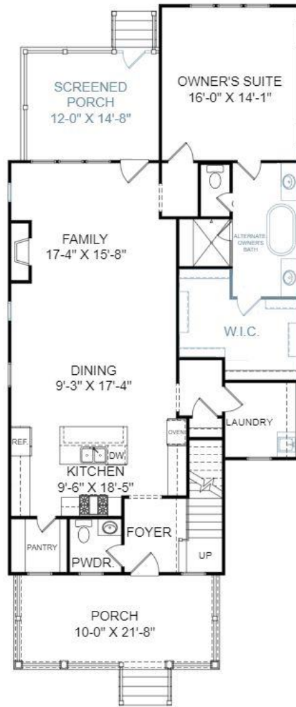
Main Level
